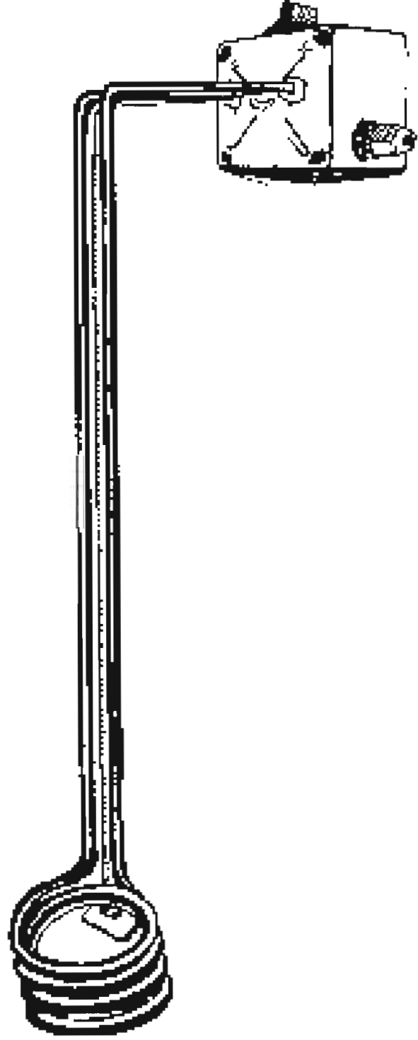
X 2128 2400W 240V 35 w/sq" FOR HEAVIER FLUIDS. COMPLETE WITH (ZCT 320) THERMOSTAT APPROXIMATE LENGTH 600mm
