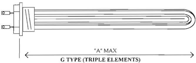
X 410 8000W 240V X 641 6000W 240V 2" BSP STEAM GENERATOR ELEMENT. SEE PAGE 34 FOR DETAILS.
